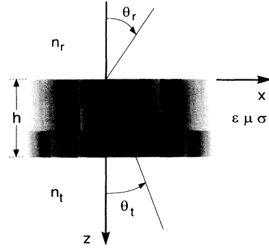
FIG. 1. Geometry for diffraction of a spatially partially coherent electromagnetic field by a structured object, which is confined between the planes z = 0 and z = h .
