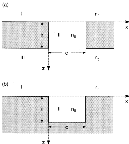
FIG. 2. Geometry for diffraction of a two-dimensional, linearly polarized, electromagnetic field by (a) a slit and (b) a groove in a perfectly conducting screen.
