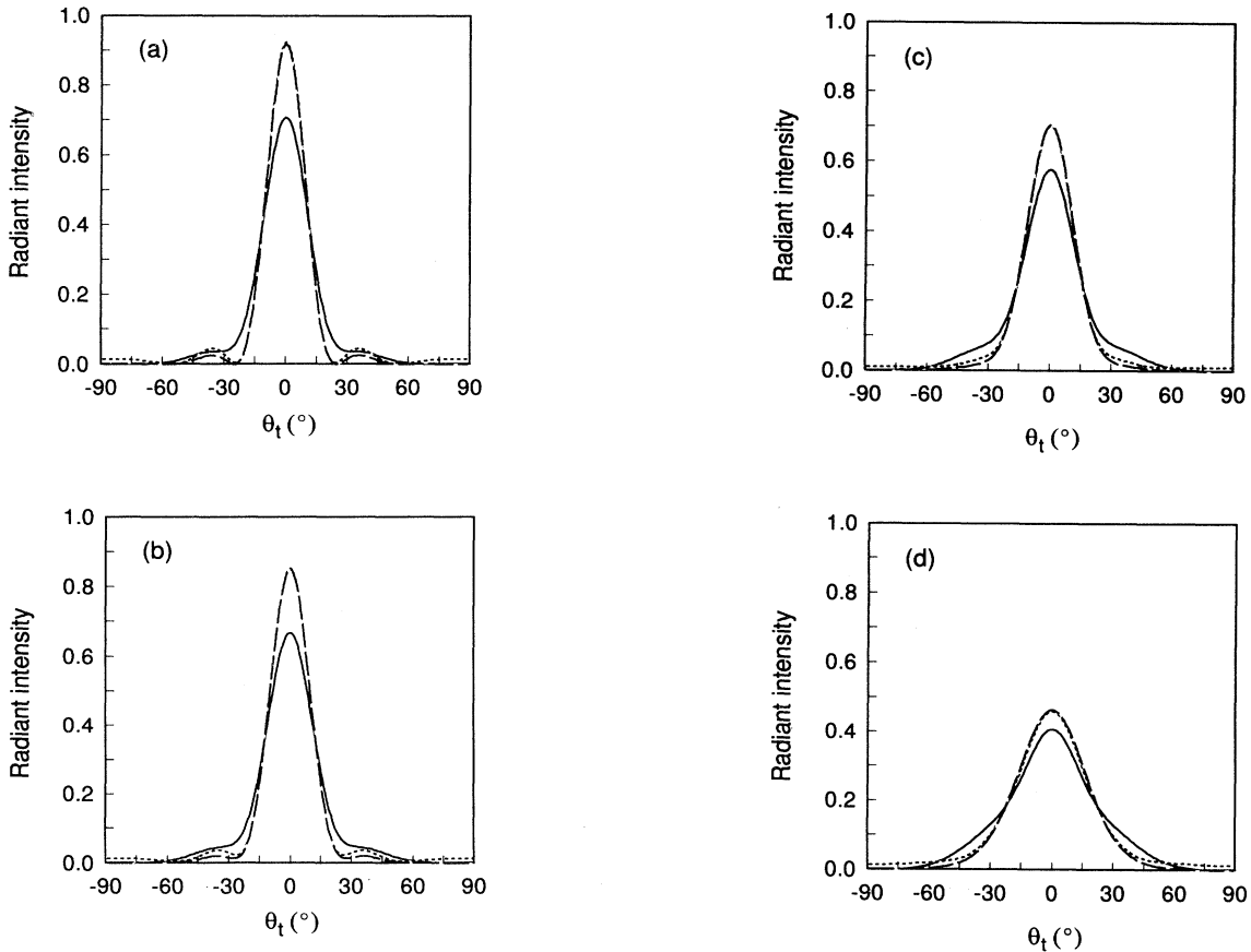
FIG. 4. Radiant intensity of a GSM field with w = 4.8\lambda diffracted by a slit of width c = 2.4\lambda and depth h = \lambda when (a) \sigma_g = \infty , (b) \sigma_g = 2.4\lambda , (c) \sigma_g = 1.2\lambda , (d) \sigma_g = 0.6\lambda . Solid curves: TE polarization. Dotted curves: TM polarization. Dashed curves: approximate results.
