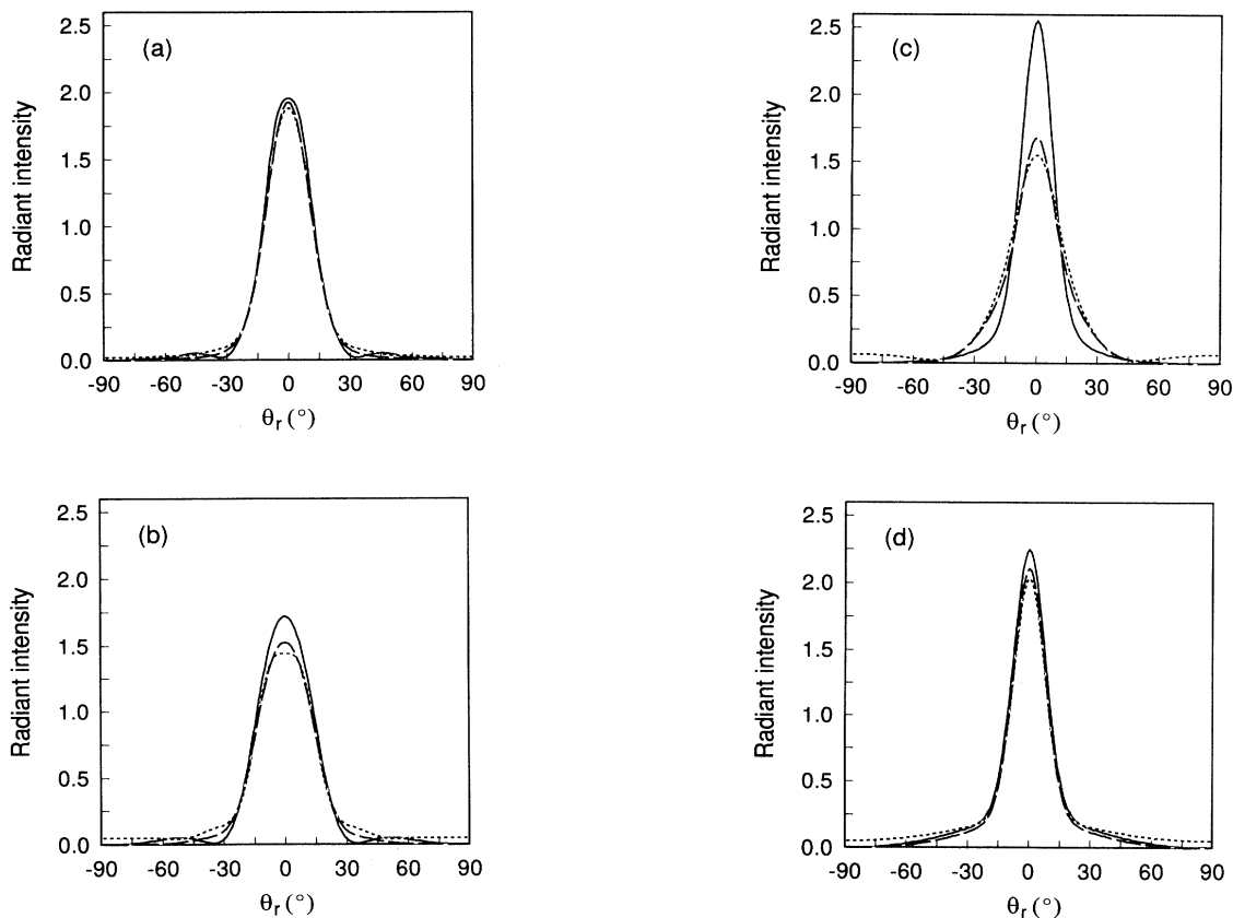
FIG. 7. Diffraction of a GSM field ( w=4.8\lambda and \sigma_g=1.2\lambda ) by a groove of depth h=1.2\lambda and width (a) c=4.8\lambda , (b) c=2.4\lambda , (c) c=1.2\lambda , (d) c=0.6\lambda . Solid curves: TE polarization. Dotted curves: TM polarization. Dashed curves: approximate results.
