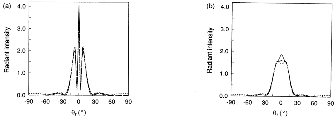
FIG. 5. Radiant intensity of a GSM field with w = 4.8\lambda diffracted by a groove of width c = 2.4\lambda and depth h = 0.2\lambda when (a) \sigma_g = \infty , (b) \sigma_g = 2.4\lambda . Solid curves: TE polarization. Dotted curves: TM polarization. Dashed curves: approximate results.
