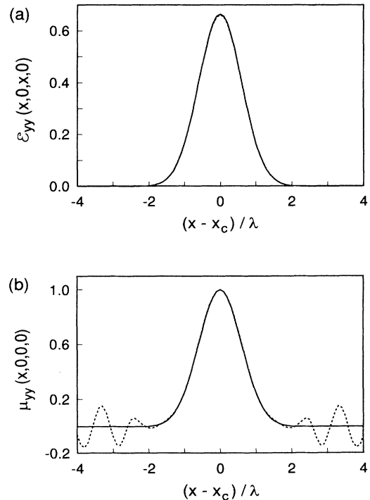
FIG. 3. (a) Distribution of electric energy density \mathcal{E}_{yy}(x, 0, x, 0) and (b) degree of coherence \mu_{yy}(x, 0, 0, 0) of a GSM field with w = 1.2\lambda , \sigma_g = 0.6\lambda (solid curve) and a field with the angular spectrum truncated by an imaging system with \mathcal{A}_{\text{num}} = 1 (dotted curve).
