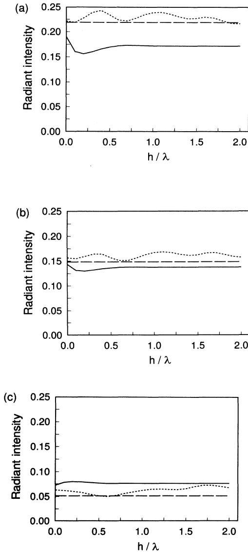
FIG. 8. Diffraction of a GSM field ( w = 4.8\lambda and \sigma_g = 1.2\lambda ) by a slit of width c = 1.2\lambda and varying depth h with radiant intensity at a polar angle (a) \theta_i = 0^\circ , (b) \theta_i = 15.67^\circ , (c) \theta_i = 30^\circ . Solid curves: TE polarization. Dotted curves: TM polarization. Dashed curves: approximate results.
