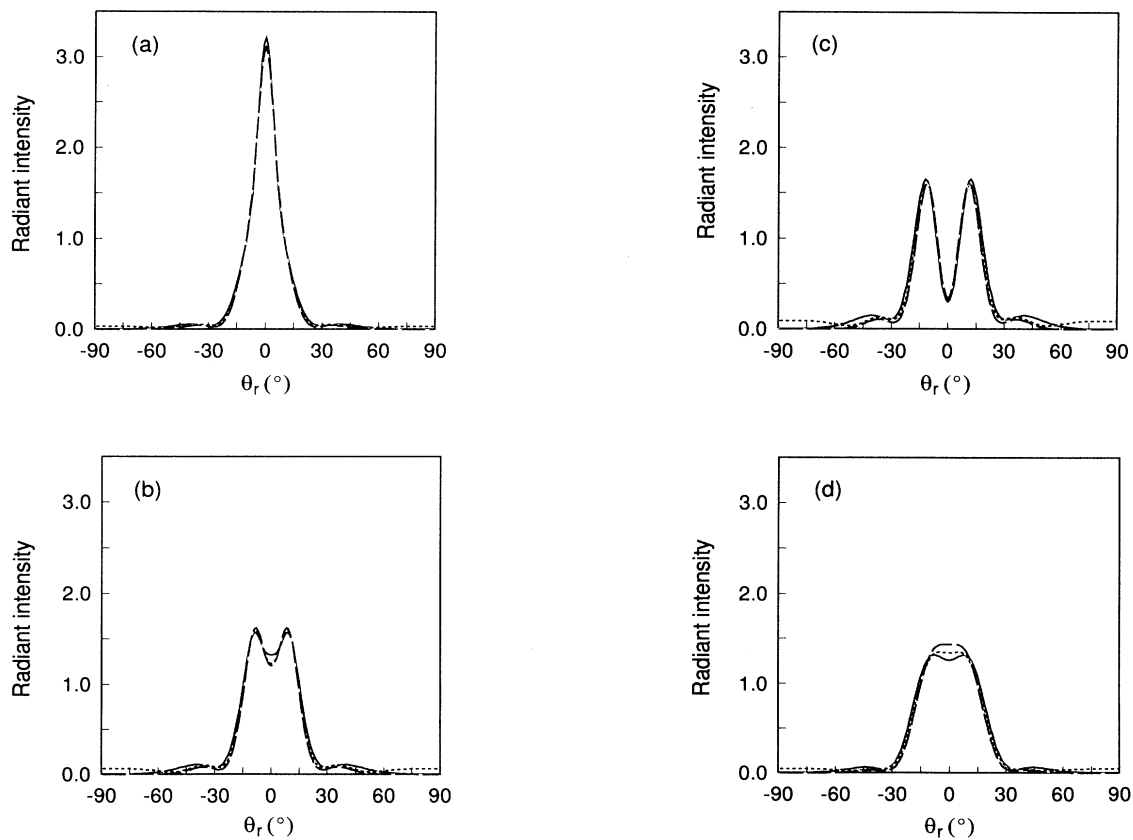
FIG. 6. Diffraction of a GSM field by a groove of width c = 2.4\lambda and depth h = 0.25\lambda , when \sigma_g = 2.4\lambda and (a) w = 9.6\lambda , (b) w = 4.8\lambda , (c) w = 2.4\lambda , (d) w = 1.2\lambda . Solid curves: TE polarization. Dotted curves: TM polarization. Dashed curves: approximate results.
